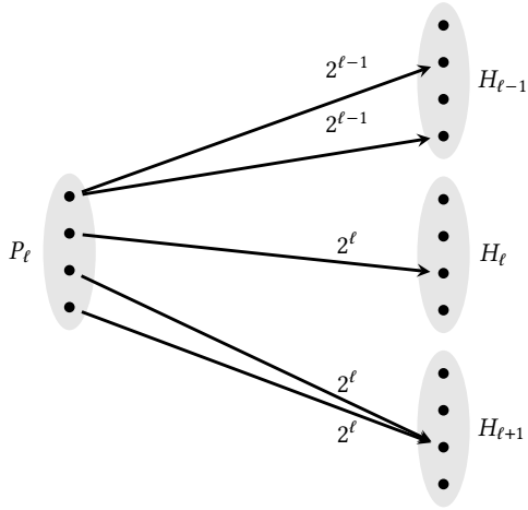
Figure 5.1: Possible ways pigeons in P_\ell can fly.
