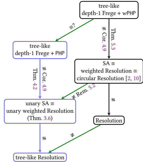
Figure 1.1: The p-simulations for SA. The notation P \rightarrow Q means that the proof system P p-simulates the proof system Q . The p-simulations are annotated with “ \neq ” if the p-simulation is known to be strict, or with “ \equiv? ” whenever it is an open question if the p-simulation is strict or not. An arrow \rightarrow means the p-simulation is trivial. The color \bullet is used to visually differentiate the results for the proof systems with unary weights/coefficients.
