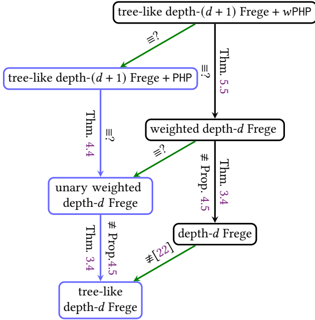
Figure 1.3: The p-simulations for weighted depth- d Frege.
